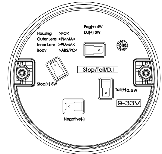
Rückansicht LED Einsatz rear view LED unit
